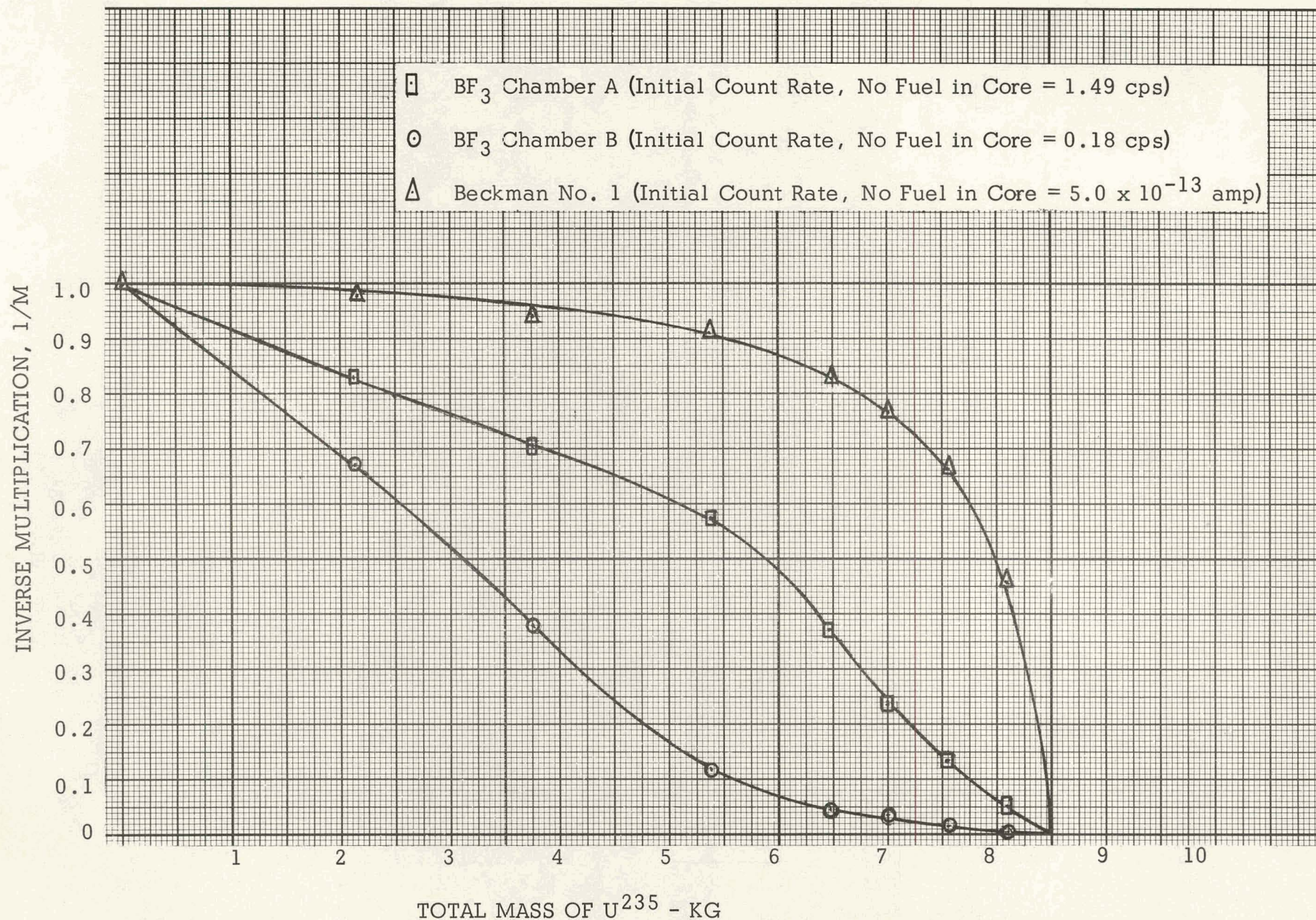
Figure 3.2. Inverse Multiplication Vs Total \text{U}^{235} In Core PM-2A Core II ZPE VI
