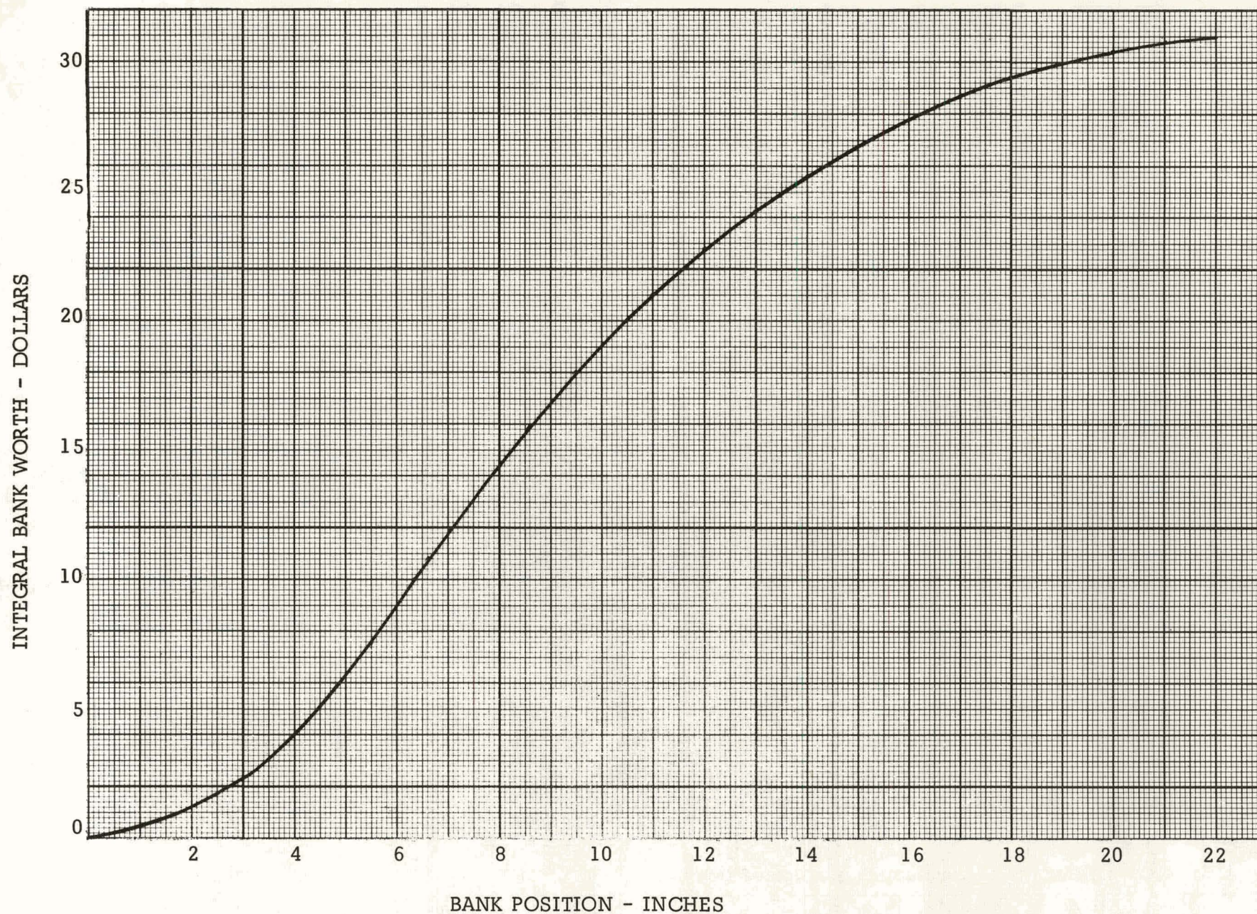
Figure 5.3. Integral Bank Worth Vs Core Reactivity For PM-2A Cores - PM-2A Core II ZPE VI
