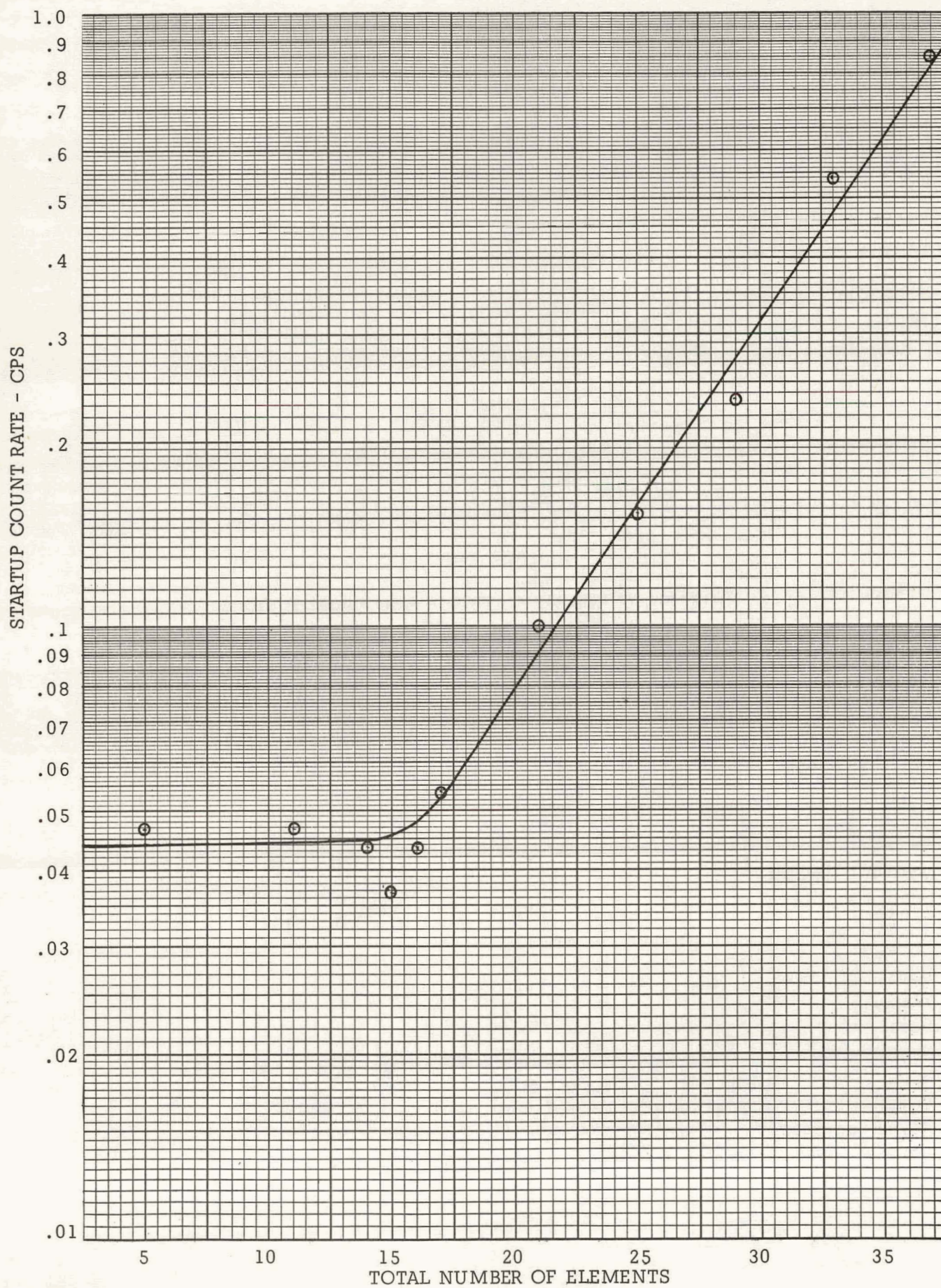
42 Figure 4.2. Startup Channel Count Rate Vs Core Loading - PM-2A Core II ZPE VI
