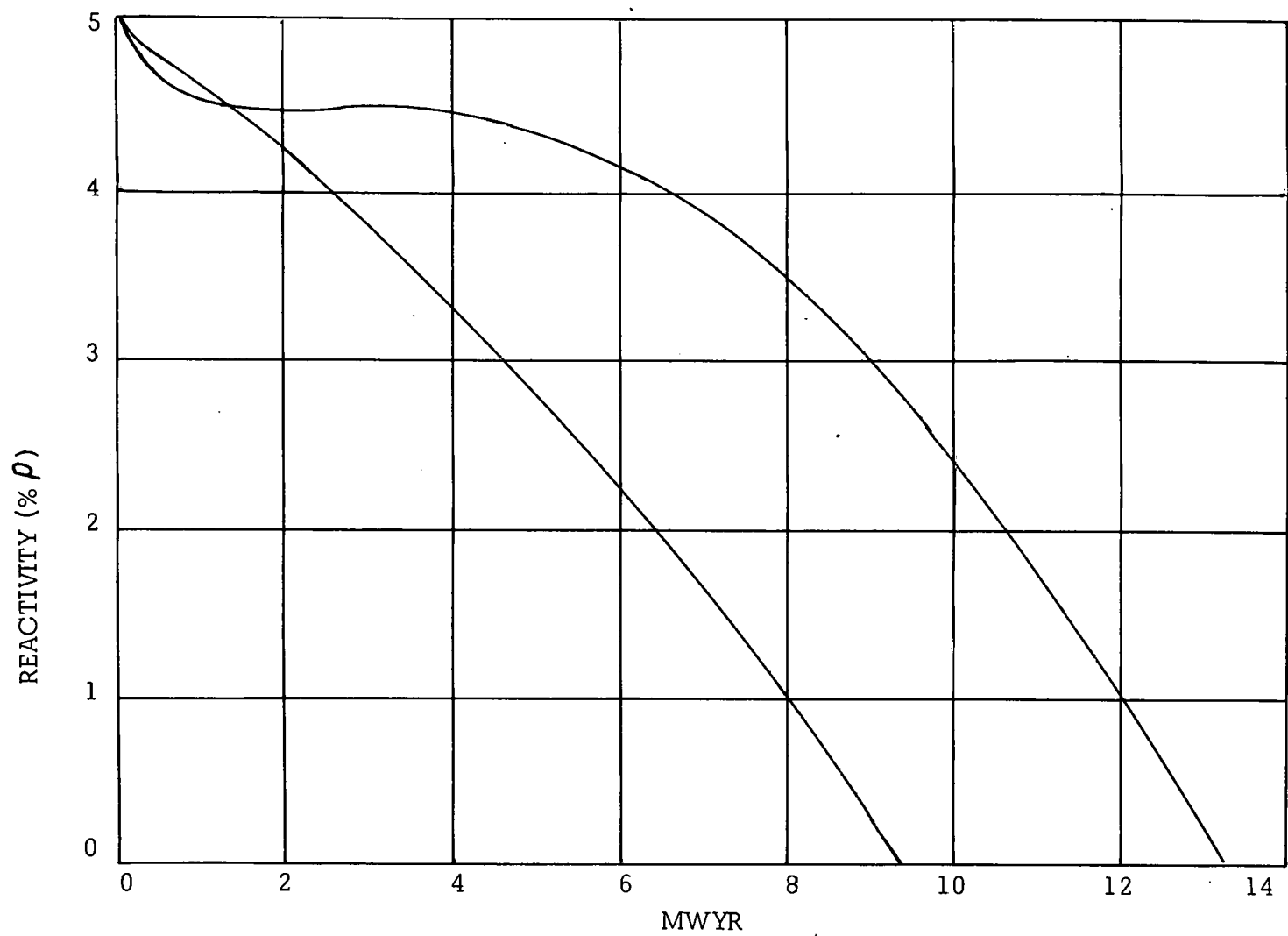
Figure 5.5. PM-2A Core I Uniform and Non-Uniform Burnup PM-2A Core II ZPE VI
