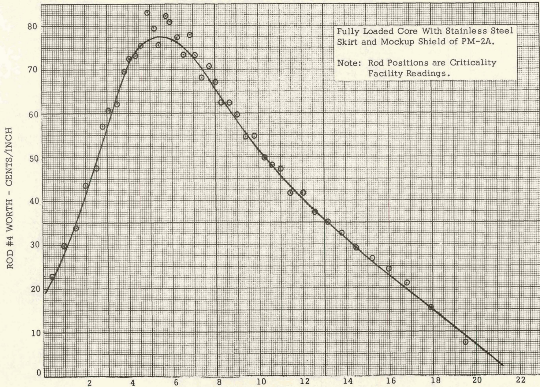
Figure 3.7. Rod #4 Calibration Curve Using B-10 Absorber - PM-2A Core II ZPE IV
