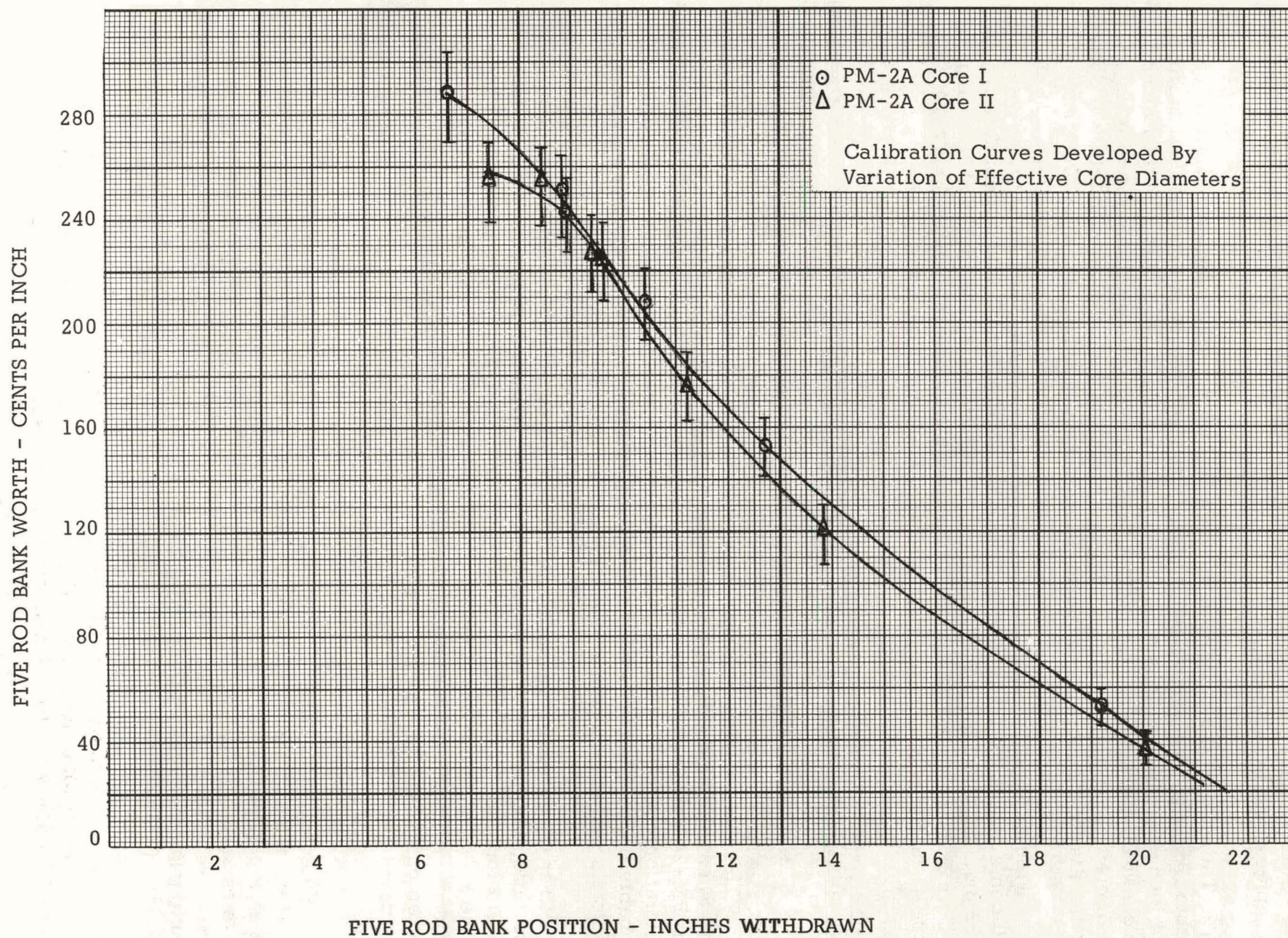
Figure 5.1. Bank Worth Vs Bank Position - PM-2A Core I and Core II ZPE VI
