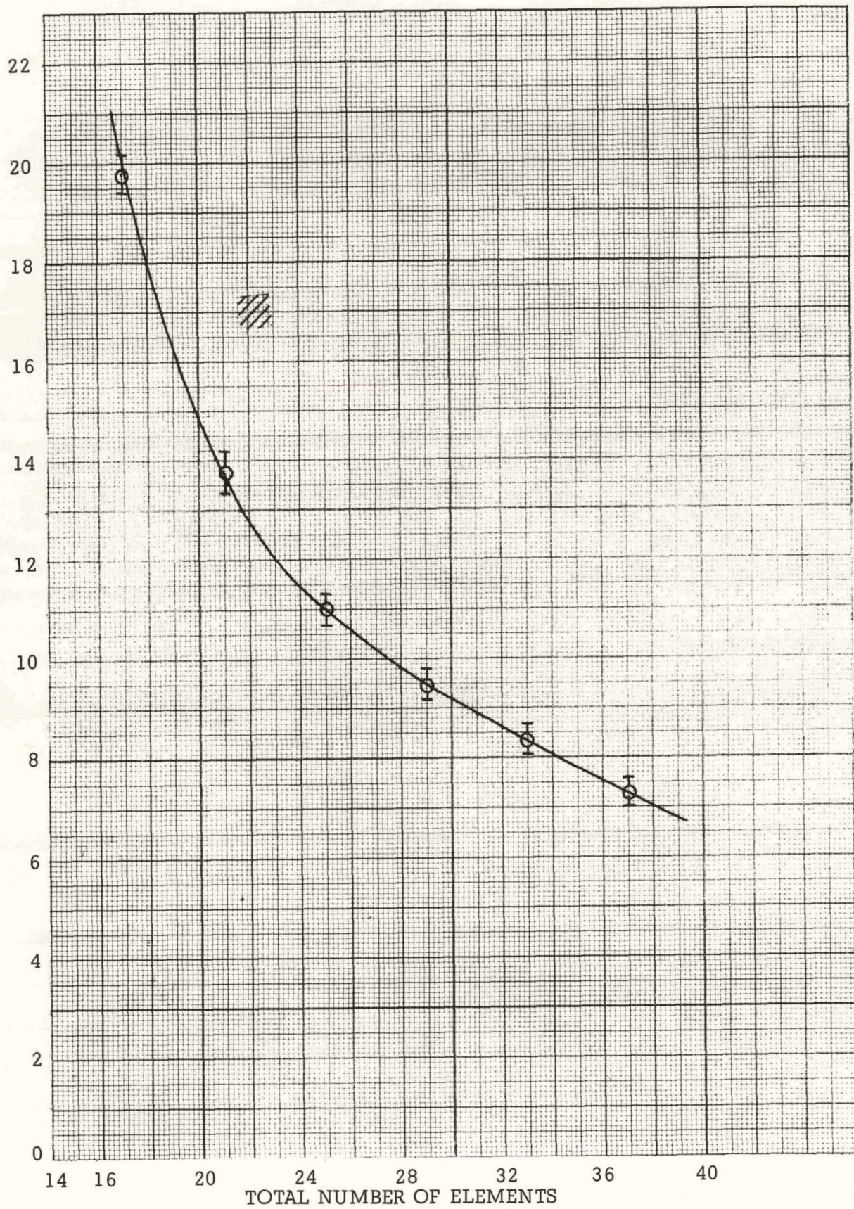
Figure 3.5. Five Rod Critical Bank Position Vs Total Number of Elements For Cold Approach To Operational Loading - PM-2A Core II ZPE VI
